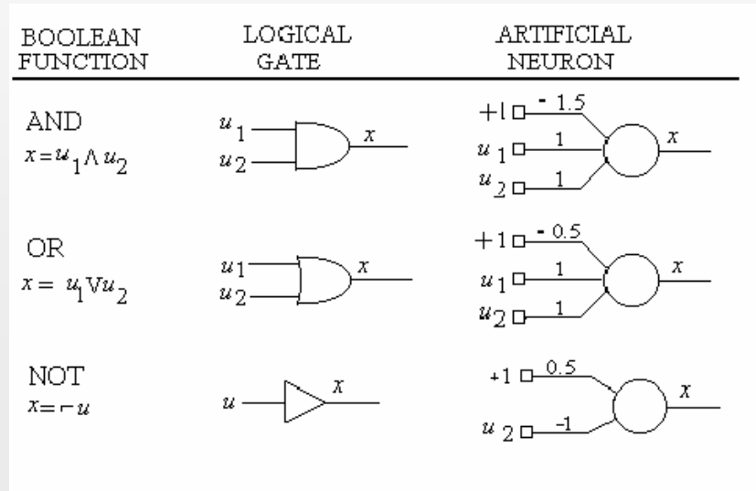
Figure 1.8. Implementation of Boolean functions by artificial neuron
