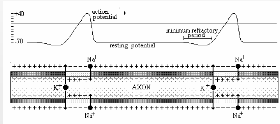
Figure 1.4. The action potential on axon
