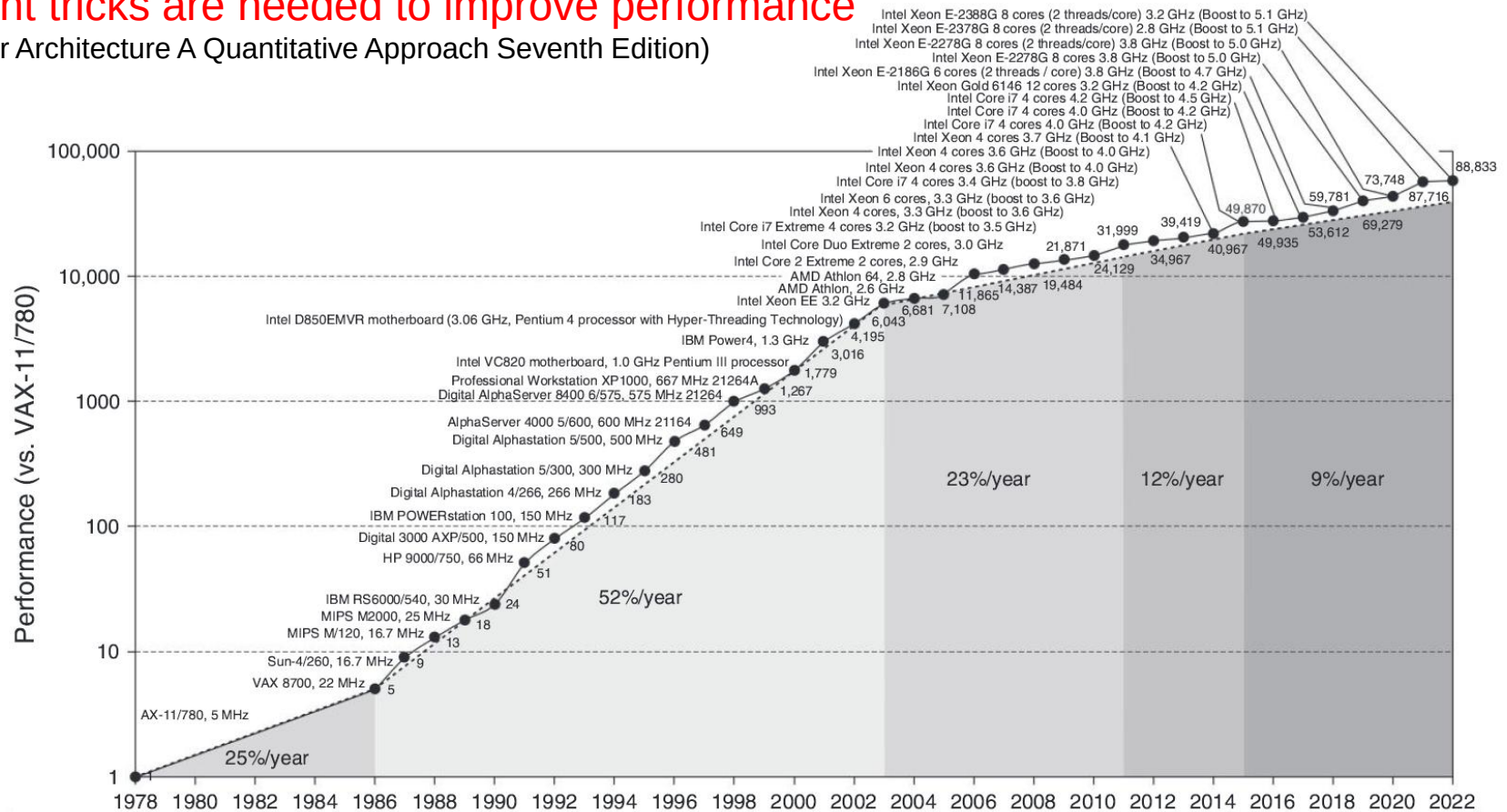
Figure 1.1 Growth in processor performance over 45 years. This chart plots program performance relative to the VAX 11/780 as measured by the SPEC
