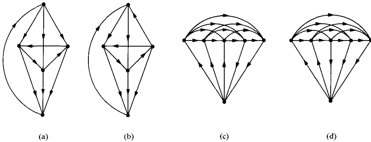
Fig. 16.8. Two pairs of nonreconstructable strong tournaments.
