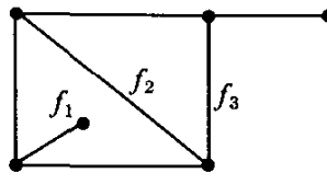
Fig. 11.2. A plane graph.
