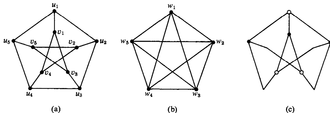
Fig. 11.12. Nonplanarity of the Petersen graph.
