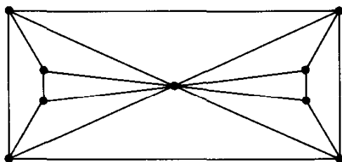
Fig. 12.9. A uniquely 3-colorable planar graph.
