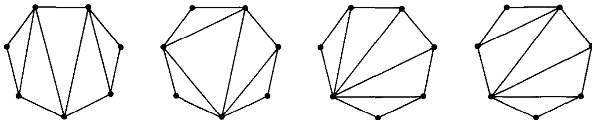
Fig. 11.9. The four maximal outerplanar graphs with seven points.
