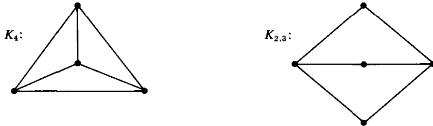
Fig. 11.7. The forbidden graphs for outerplanarity.
