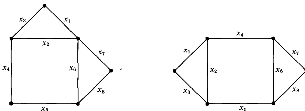
Fig. 13.3. Two graphs with the same cycle matrix.
