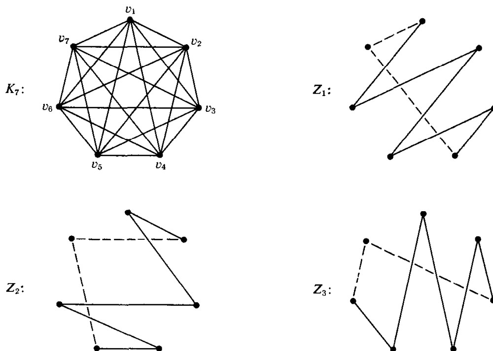
Fig. 9.4. A 2-factorization of K_7 .
