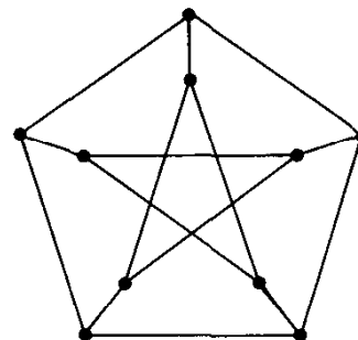
Fig. 9.6. The Petersen graph.
