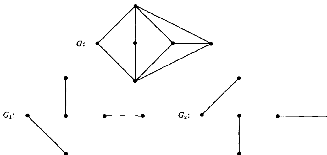
Fig. 9.2. Two 1-factors of a block.
