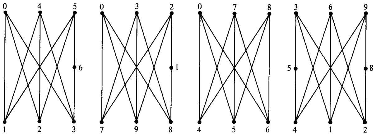
Fig. 11.19. Four nonplanar subgraphs of K_{10} .
