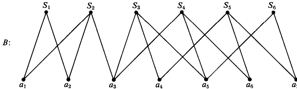
Fig. 5.9. A bipartite graph illustrating Hall's Theorem.
