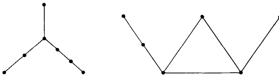
Fig. 14.1. Two identity graphs.
