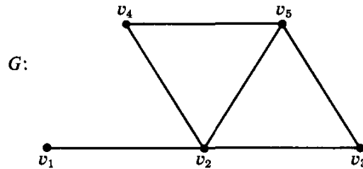
Fig. 2.9. A graph to illustrate walks.
