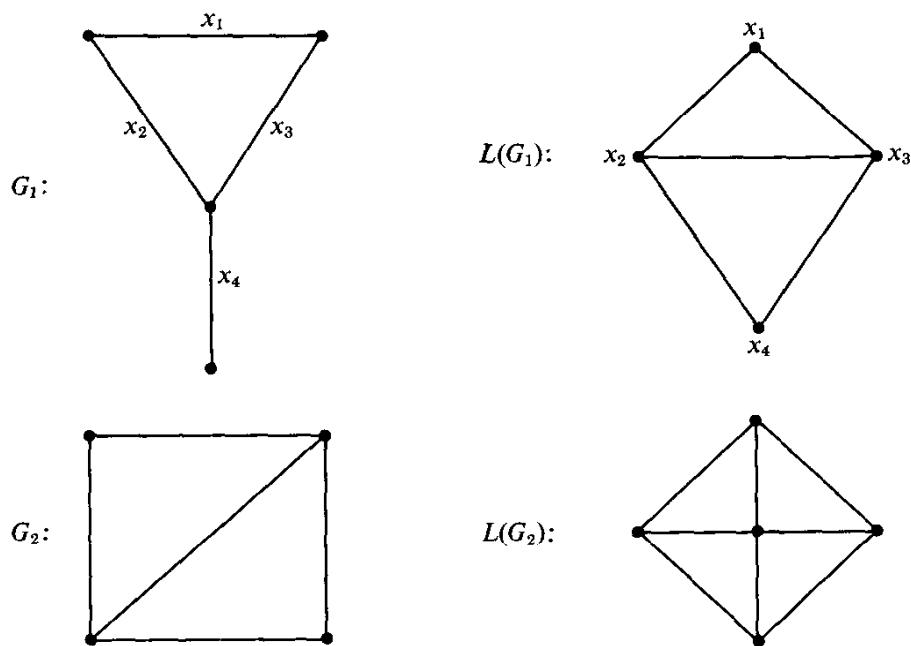
Fig. 8.1. Graphs and their line graphs.
