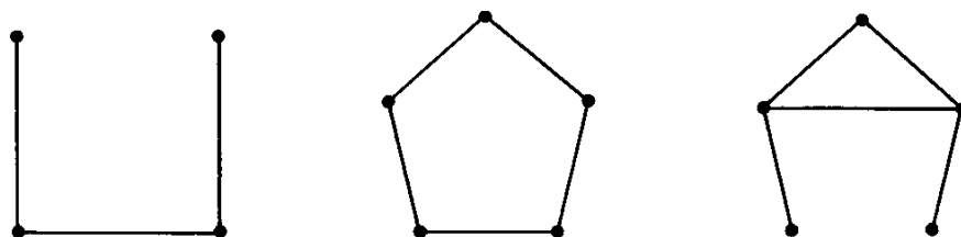
Fig. 2.13. The smallest nontrivial self-complementary graphs.
