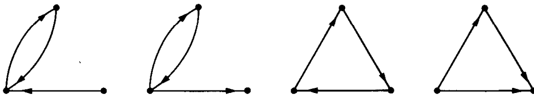
Fig. 2.4. The digraphs with three points and three arcs.
