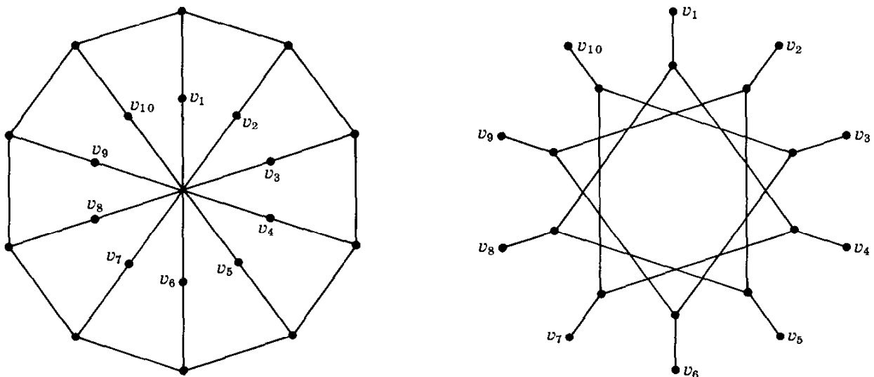
Fig. 14.13. The 8-cage is the union of the above subgraphs as labeled.
