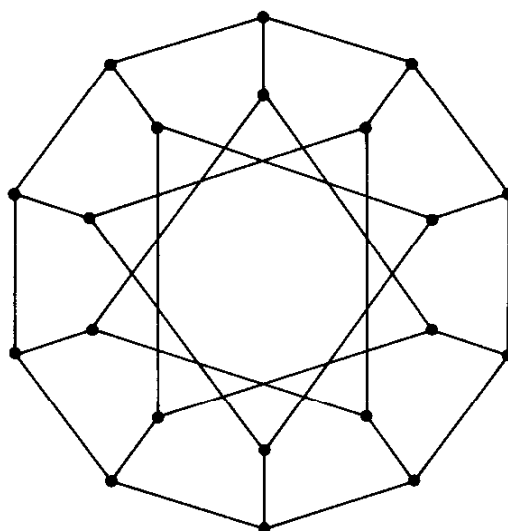
Fig. 14.14. Another 3-unitransitive graph.
