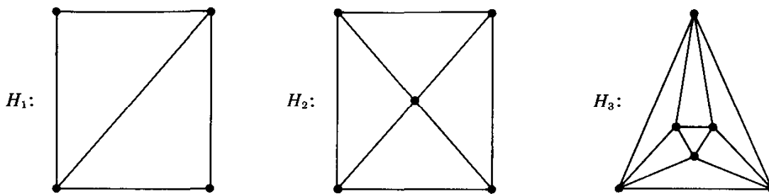
Fig. 8.4. Three line graphs.
