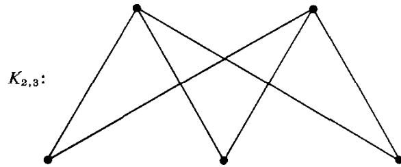
Fig. 14.10. A line-regular line-symmetric graph.
