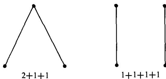
Fig. 6.1. The graphical partitions of 4.
