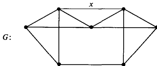
Fig. 12.10. A critical graph which is not line-critical.
