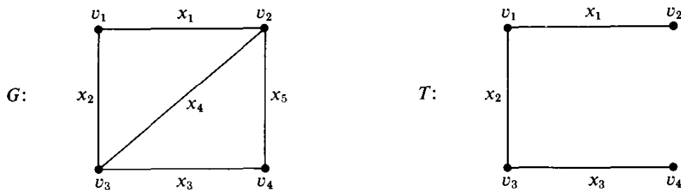
Fig. 13.4. A graph and a spanning tree.
