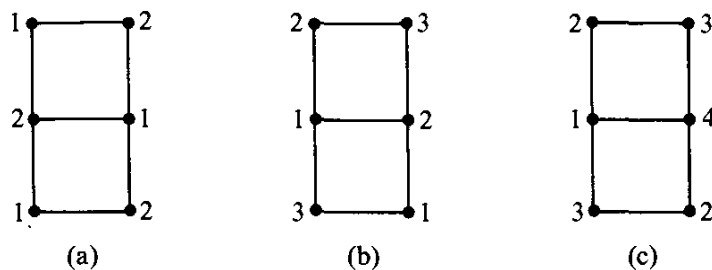
Fig. 12.1. Three colorings of a graph.
