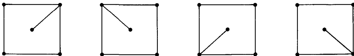
Fig. 13.5. The new circuits in the whirl of W_5 .
