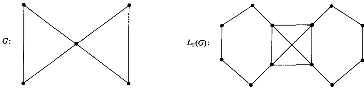
Fig. 8.10. Still another counterexample.
