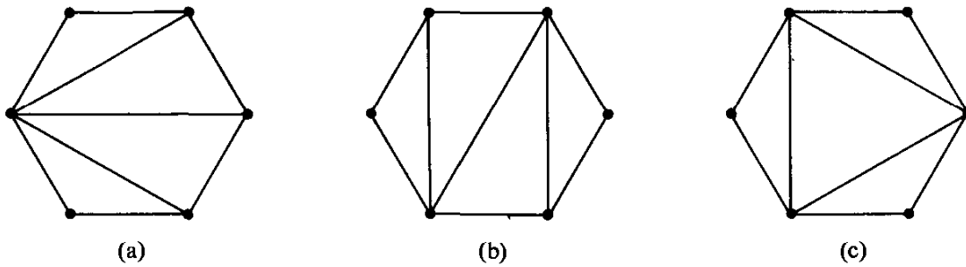
Fig. 11.6. Three maximal outerplanar graphs.
