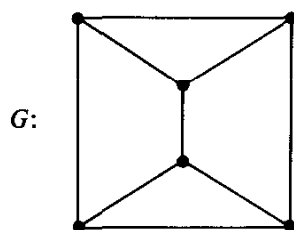
Fig. 12.7. A counterexample to the converse of Theorem 12.16.
