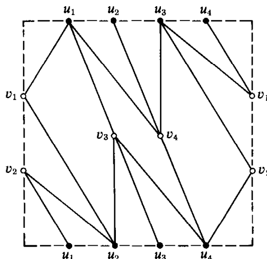
Fig. 11.18. A toroidal embedding of K_{4,4} .
