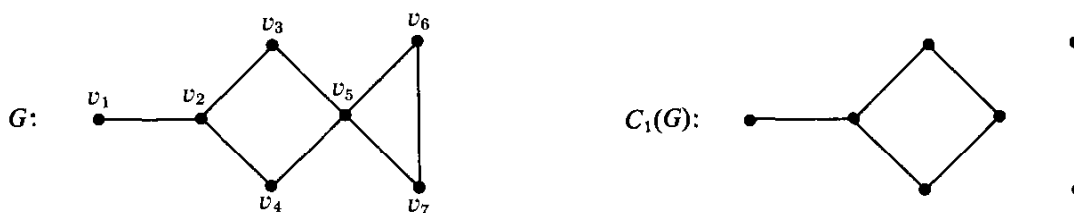
Fig. 10.3. A graph and its line-core.
