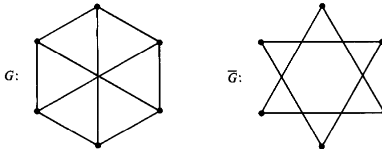
Fig. 2.12. A graph and its complement.
