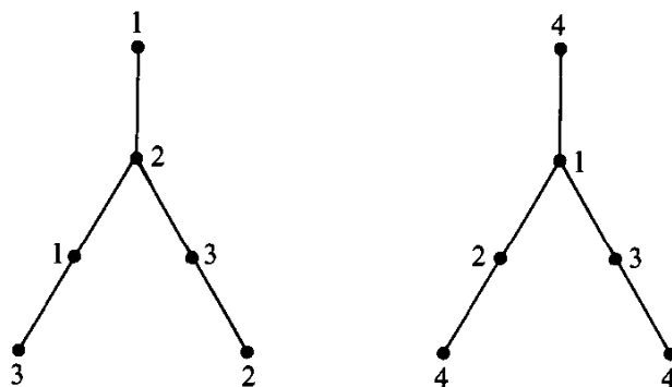
Fig. 12.12. Two complete colorings of a graph.
