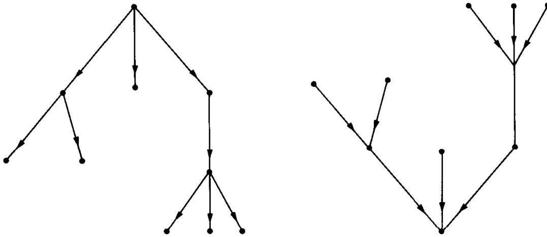
Fig. 16.2. An out-tree and the converse in-tree.
