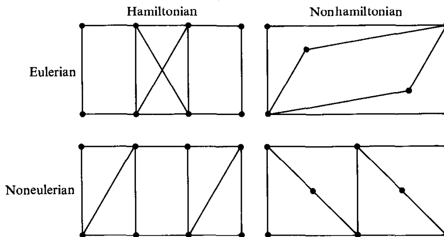
Fig. 7.5. Eulerian and/or hamiltonian graphs.
