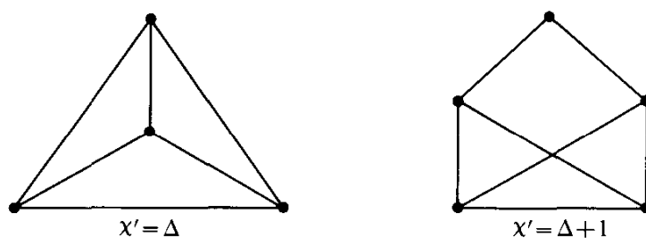
Fig. 12.5. The two values for the line-chromatic number.
