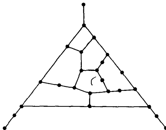
Fig. 2.20. A counterexample for Exercise 2.10.
