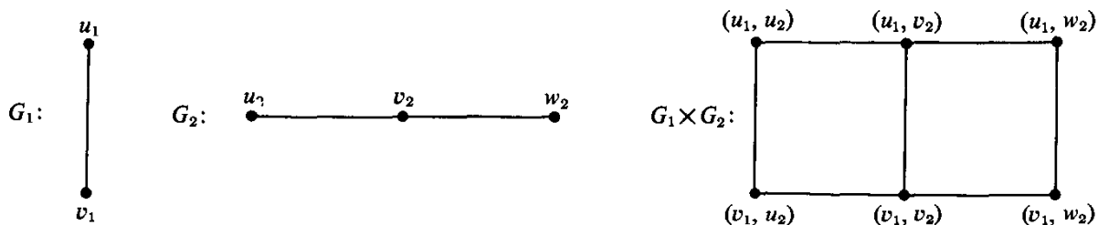
Fig. 2.17. The product of two graphs.
