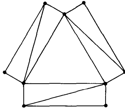
Fig. 14.7. A smallest graph whose group is C_3 .
