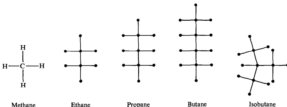
Fig. 1.4. The smallest saturated hydrocarbons.
