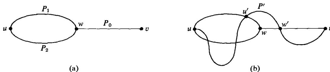
Fig. 3.2. Paths in blocks.
