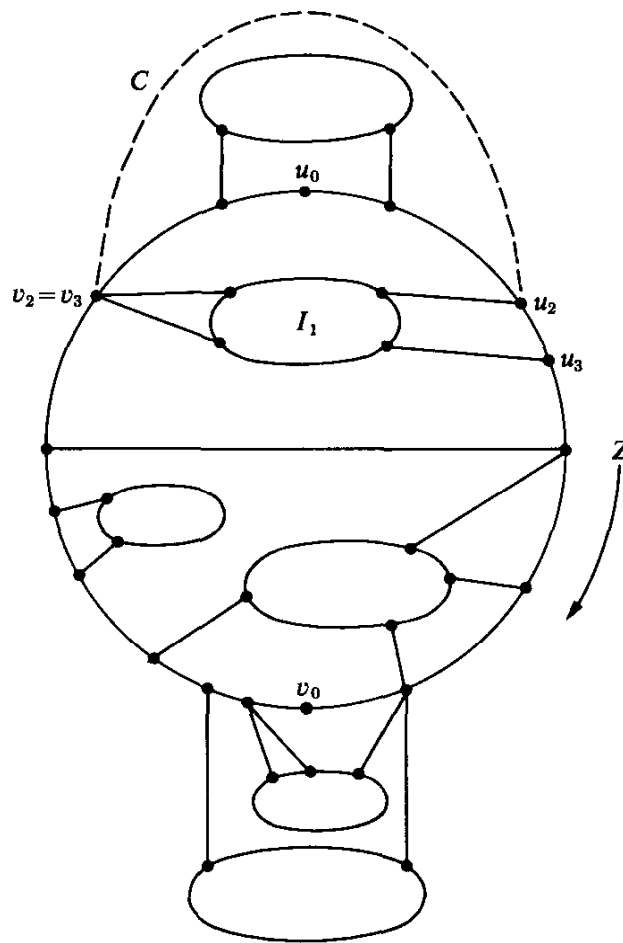
Fig. 11.10. Separating cycle Z illustrating lemma.
