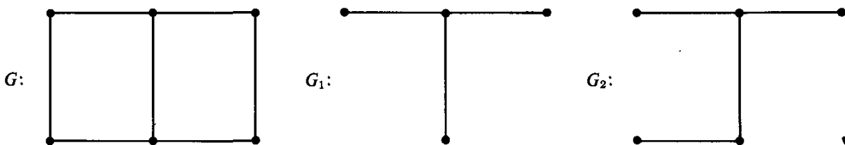
Fig. 2.6. A graph and two subgraphs.
