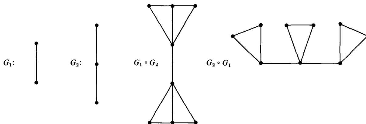
Fig. 14.3. Two graphs and their two coronas.
