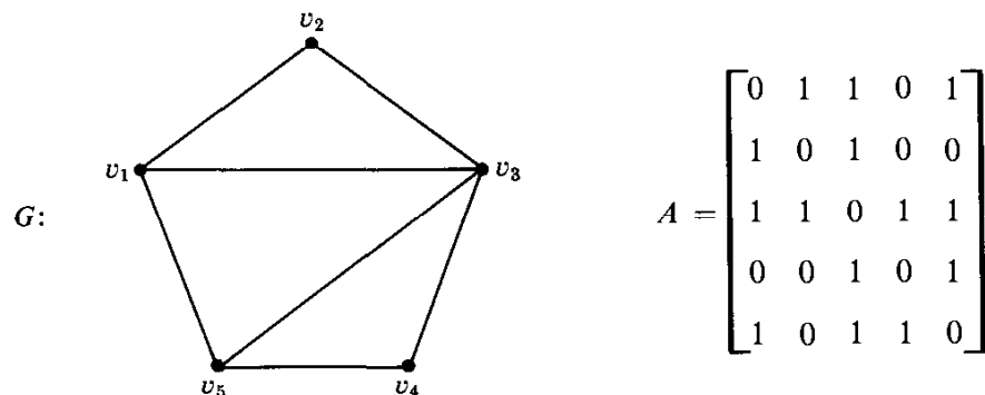
Fig. 13.1. A labeled graph and its adjacency matrix.
