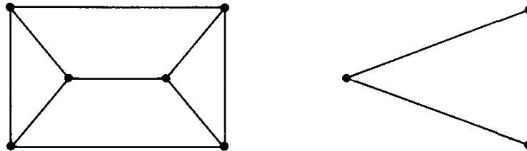
Fig. 14.8. A point-symmetric and a line-symmetric graph.
