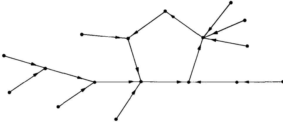
Fig. 16.3. A weak functional digraph.
