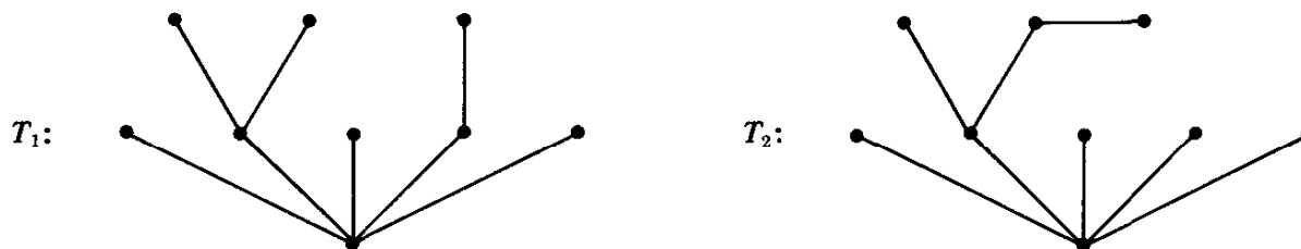
Fig. 6.3. Two trees with the same partition.
