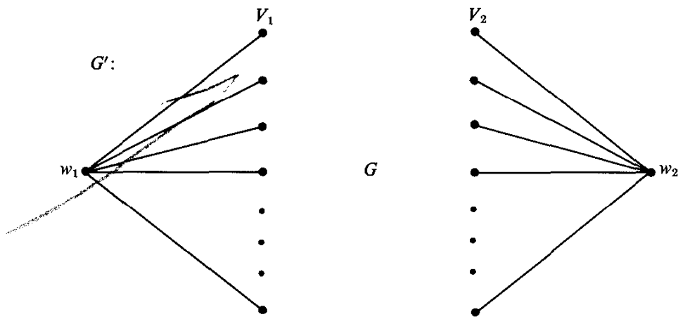
Fig. 5.6. Construction of G' .
