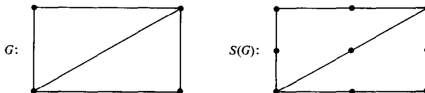
Fig. 8.7. A graph and its subdivision graph.
