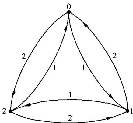
Fig. 14.4. The color graph of the cyclic group C_3 .
