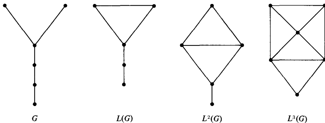
Fig. 8.12. A sequence of iterated line graphs.
