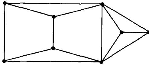
Fig. 5.4. A graph with two 3-components which meet in two points.
