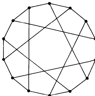
Fig. 14.11. The Heawood graph.
