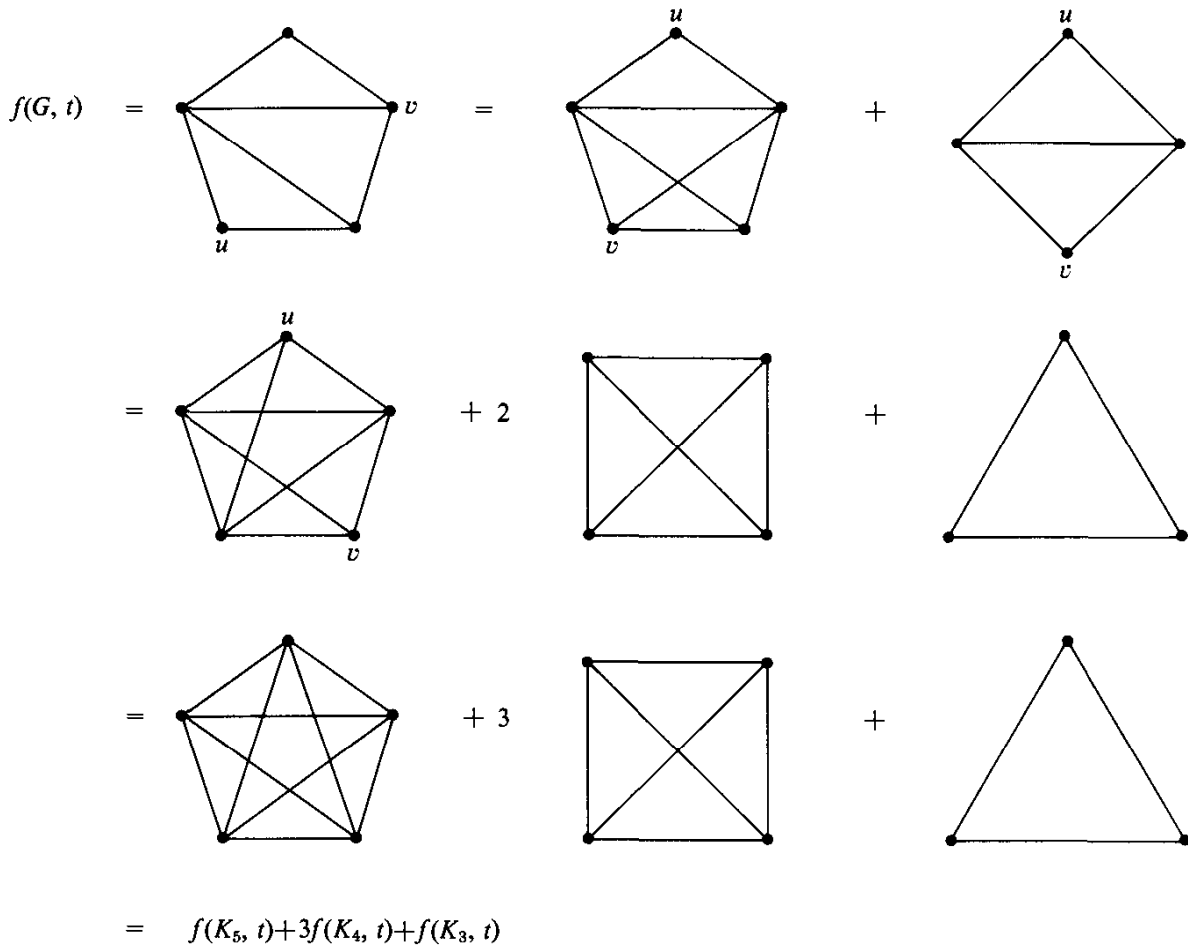
Fig. 12.15. The determination of a chromatic polynomial.
