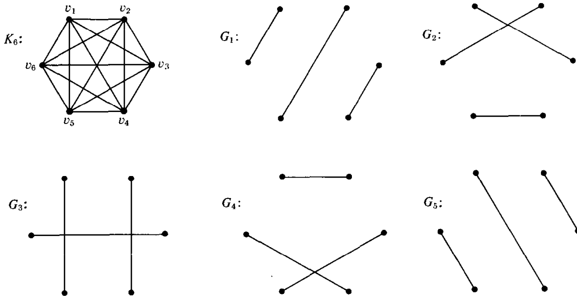
Fig. 9.1. A 1-factorization of K_6 .
