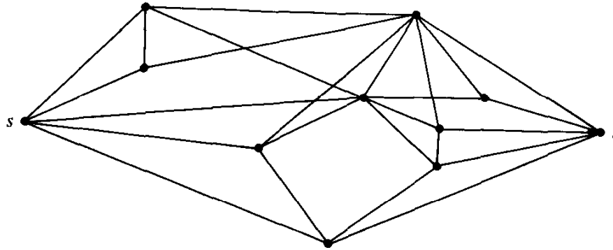
Fig. 5.5. A graph illustrating Menger's Theorem.
