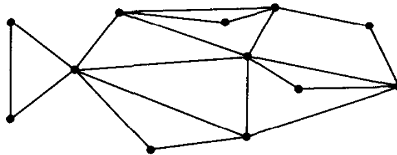
Fig. 7.1. An eulerian graph.
