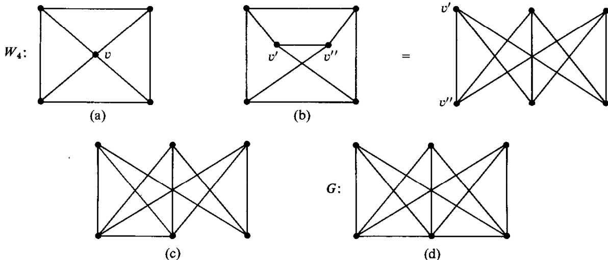
Fig. 5.3. Demonstration that a graph is 3-connected.
