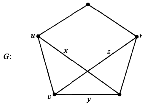
Fig. 2.2. A graph to illustrate adjacency.
