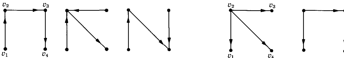
Fig. 16.5. Spanning in-trees and out-trees.
