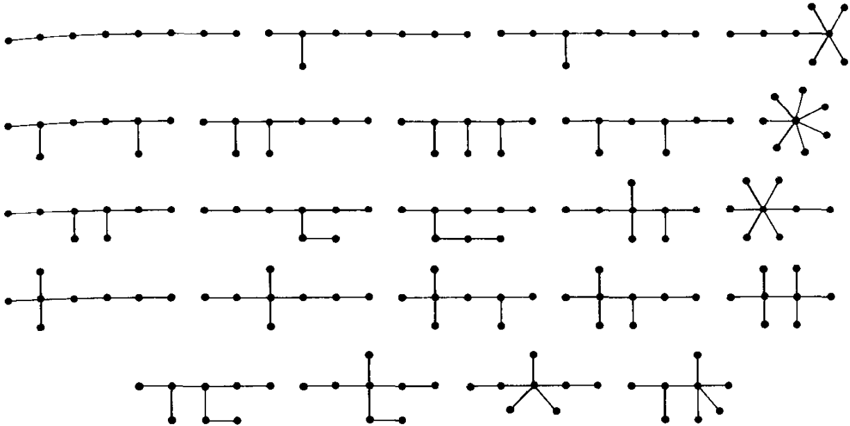
Fig. 4.1. The 23 trees with eight points.
