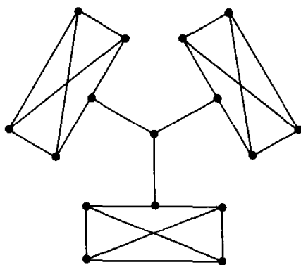
Fig. 9.5. A cubic graph with no 1-factor.
