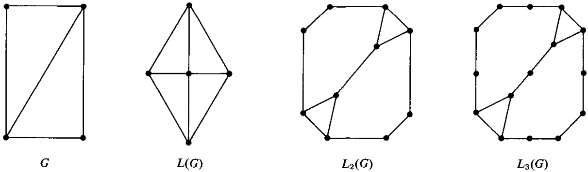
Fig. 8.11. A sequence of graphs L_n(G) .
