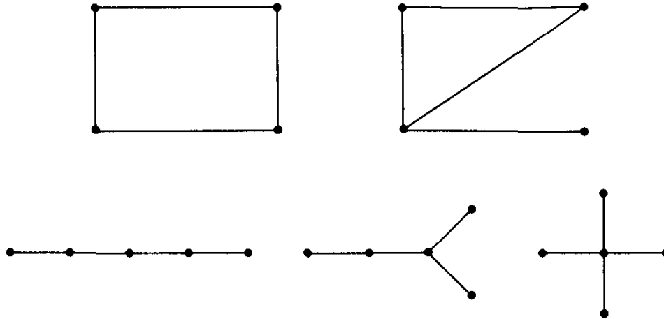
Fig. 8.2. The connected graphs with four lines.
