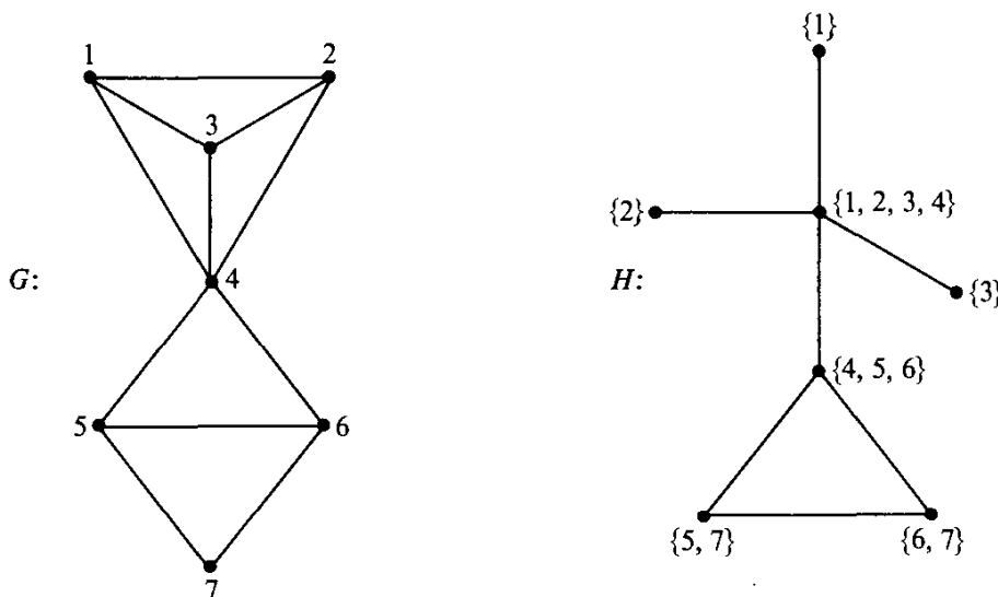
Fig. 8.5. A line graph and its graph.
