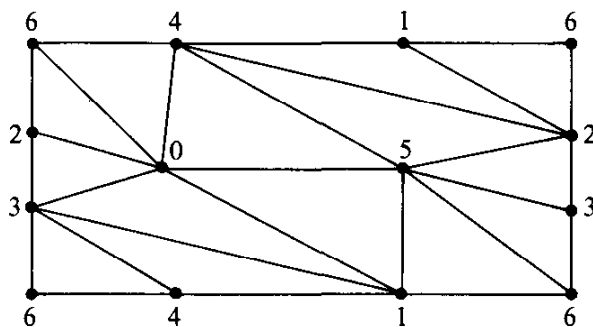
Fig. 11.17. An embedding of K_7 on the torus.
