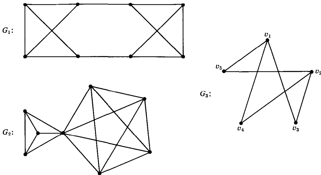
Fig. 7.3. Illustrations for the theorem of Pósa.
