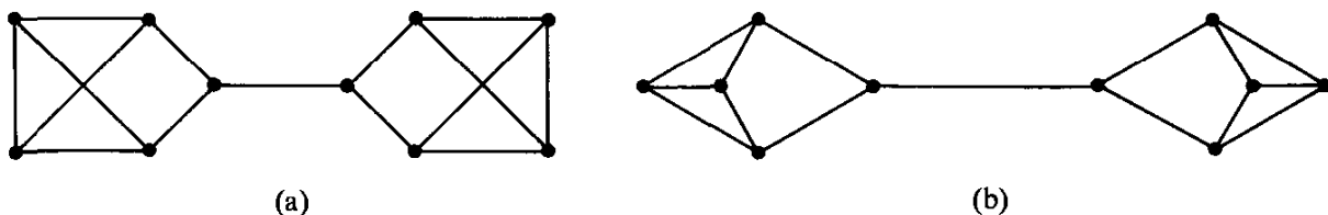
Fig. 11.1. A planar graph and an embedding.
