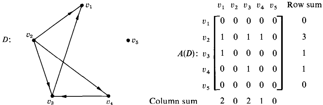
Fig. 16.4. A digraph and its adjacency matrix.
