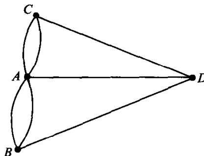
Fig. 1.2. The graph of the Königsberg Bridge Problem.
