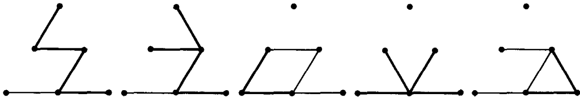
Fig. 4.8. A cocycle basis for G of Fig. 4.7.
