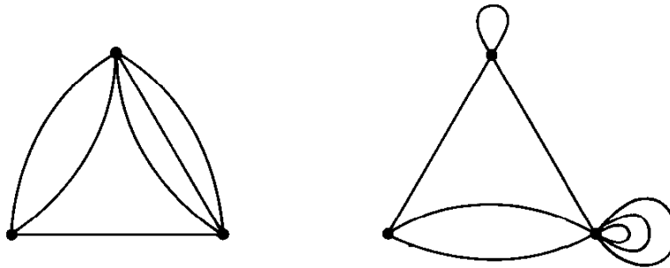
Fig. 2.3. A multigraph and a pseudograph.
