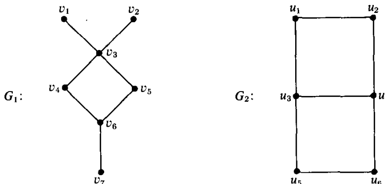
Fig. 10.4. A semi-irreducible and an irreducible graph.
