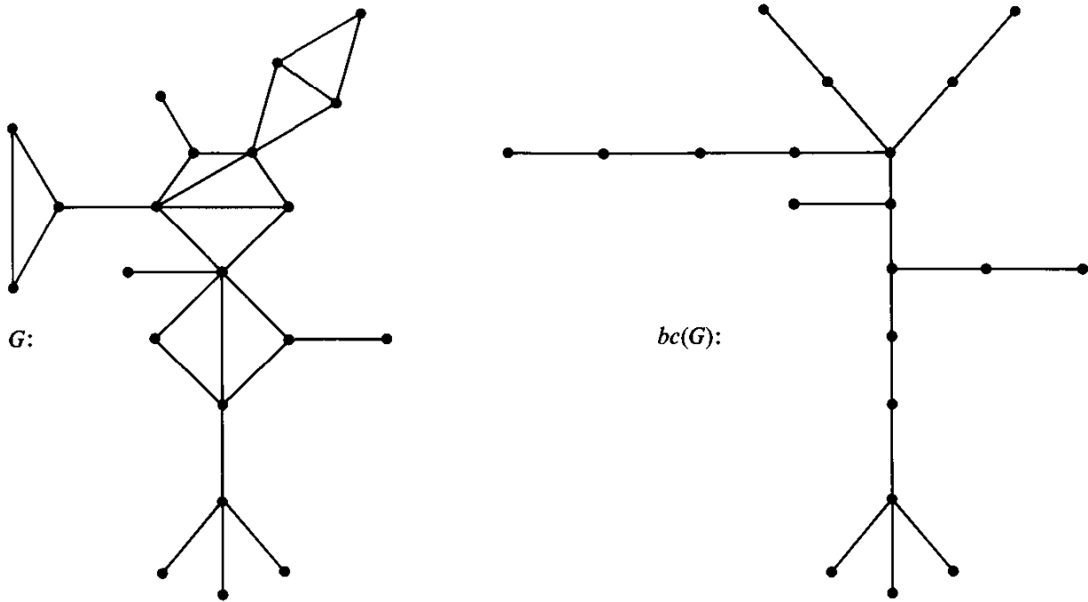
Fig. 4.5. A graph and its block-cutpoint graph.
