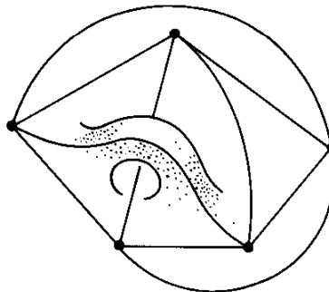
Fig. 11.16. Embedding a graph on an orientable surface.
