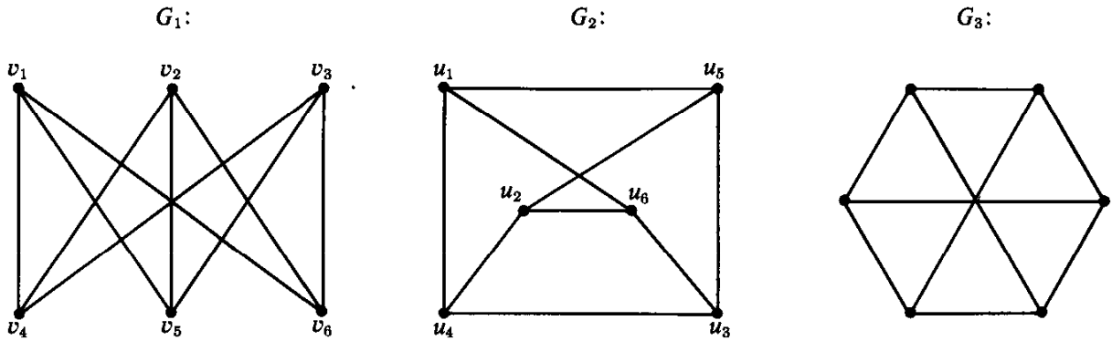
Fig. 2.5. Labeled and unlabeled graphs.
