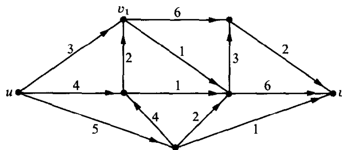
Fig. 5.7. A network with integral capacities.
