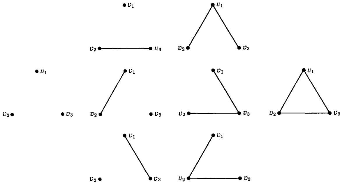
Fig. 15.1. The labeled graphs with three points.
