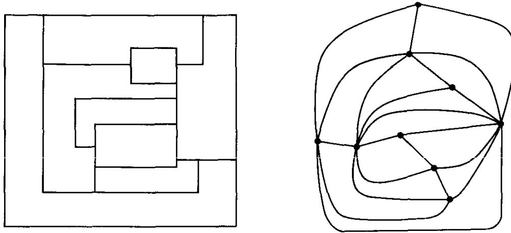
Fig. 1.6. A map and its corresponding graph.
