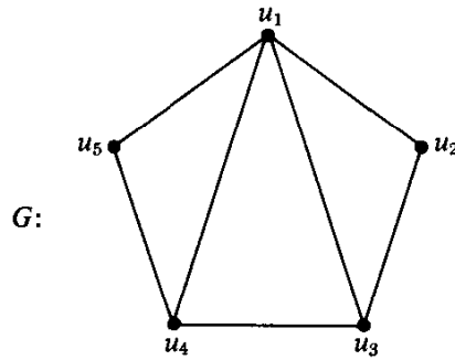
Fig. 12.6. A uniquely colorable graph.
