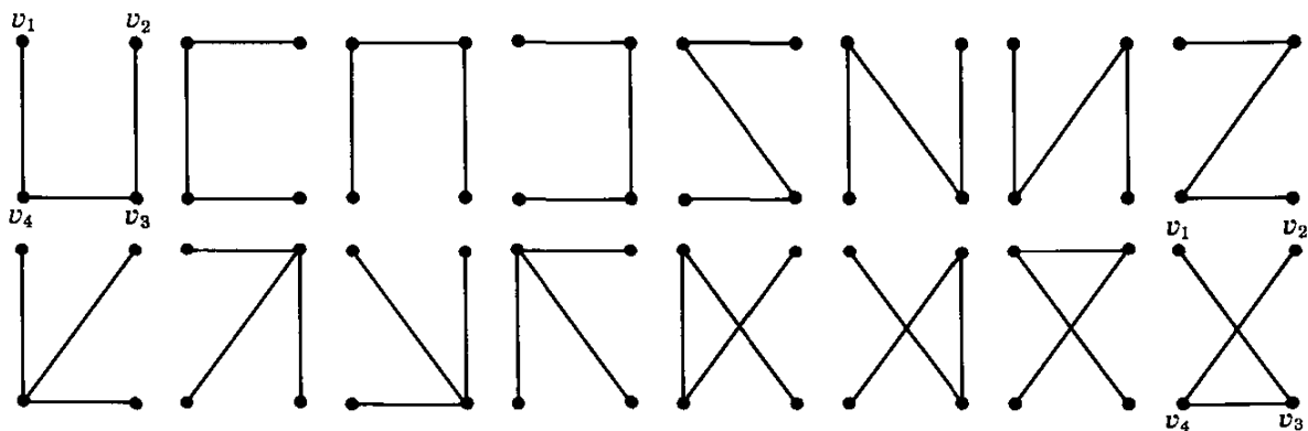
Fig. 15.2. The labeled trees with four points.
