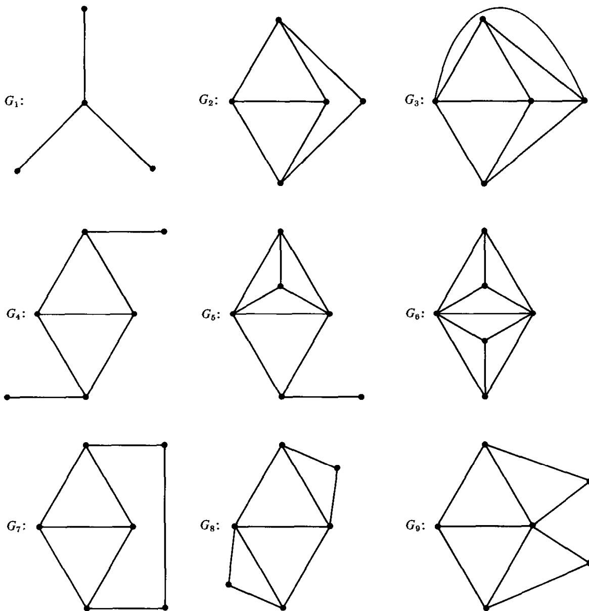
Fig. 8.3. The nine forbidden subgraphs for line graphs.
