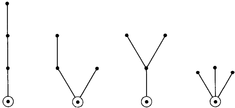
Fig. 15.4. The rooted trees with four points.
