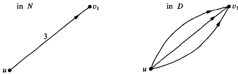
Fig. 5.8. The transformation from network to multigraph.
