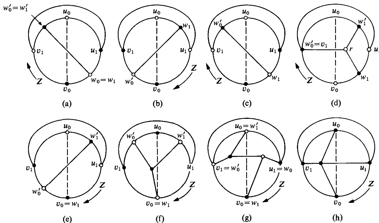
Fig. 11.11. The possibilities for nonplanar subgraphs.
