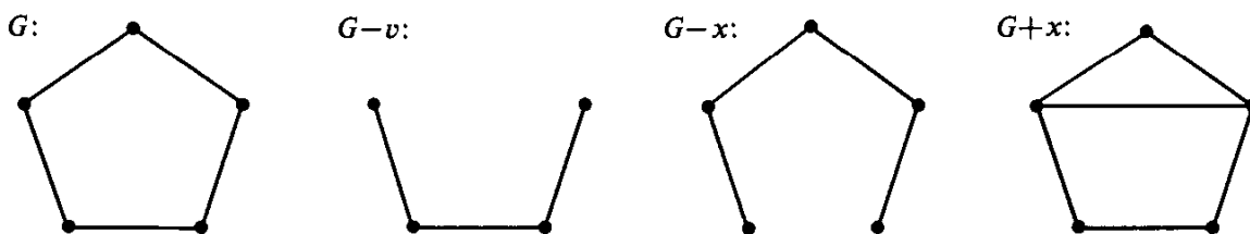
Fig. 2.8. A graph plus or minus a point or line.
