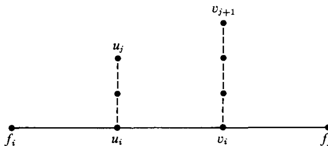
Fig. 14.5. Doubly-rooted graph to replace arc f_i f_j .
