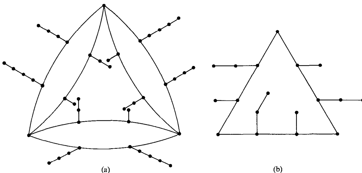
Fig. 14.6. Frucht's graph whose group is C_3 and a smaller such graph.
