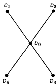
Fig. 12.14. A labeled copy of K_{1,4} .
