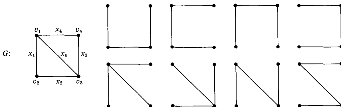
Fig. 13.2. K_4 - x and its spanning trees.
