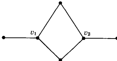
Fig. 9.3. A graph with no 1-factor.
