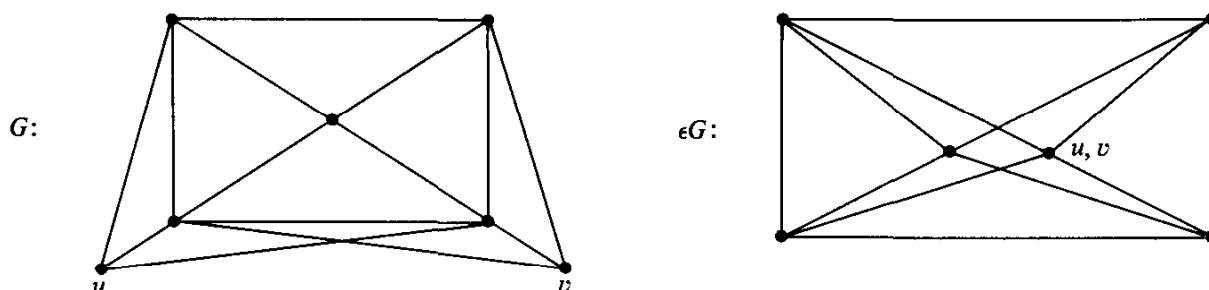
Fig. 12.13. A homomorphism which decreases \psi by 2.
