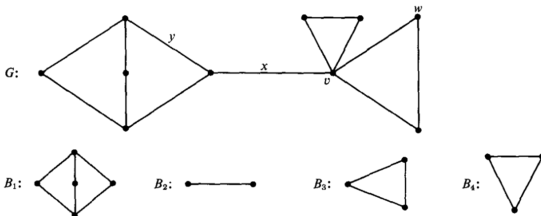
Fig. 3.1. A graph and its blocks.
