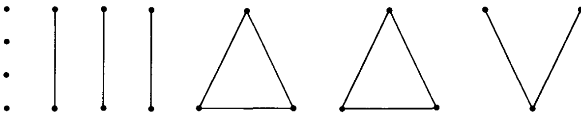
Fig. 2.10. A graph with 10 components.
