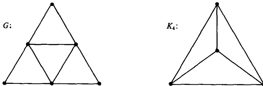
Fig. 2.15. A graph and its clique graph.
