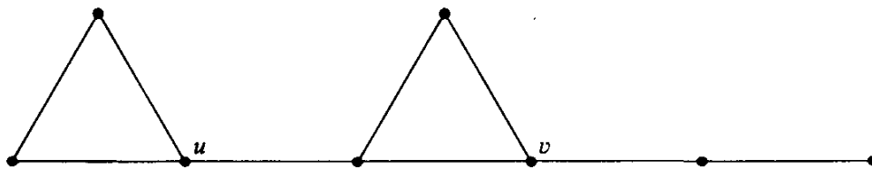
Fig. 14.9. A counterexample to a conjecture.
