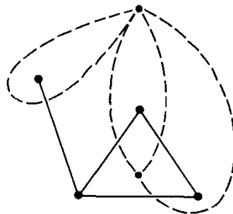
Fig. 11.13. A plane graph and its geometric dual.
