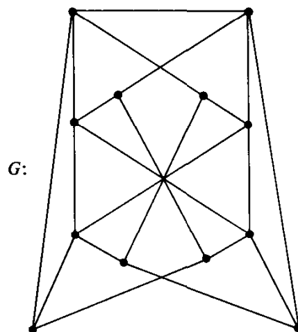
Fig. 12.8. A uniquely 3-colorable graph having no triangles.
