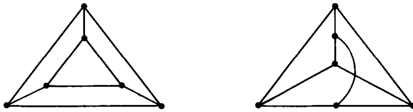
Fig. 2.11. The cubic graphs with six points.
