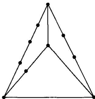
Fig. 11.8. A homeomorph of K_4 .
