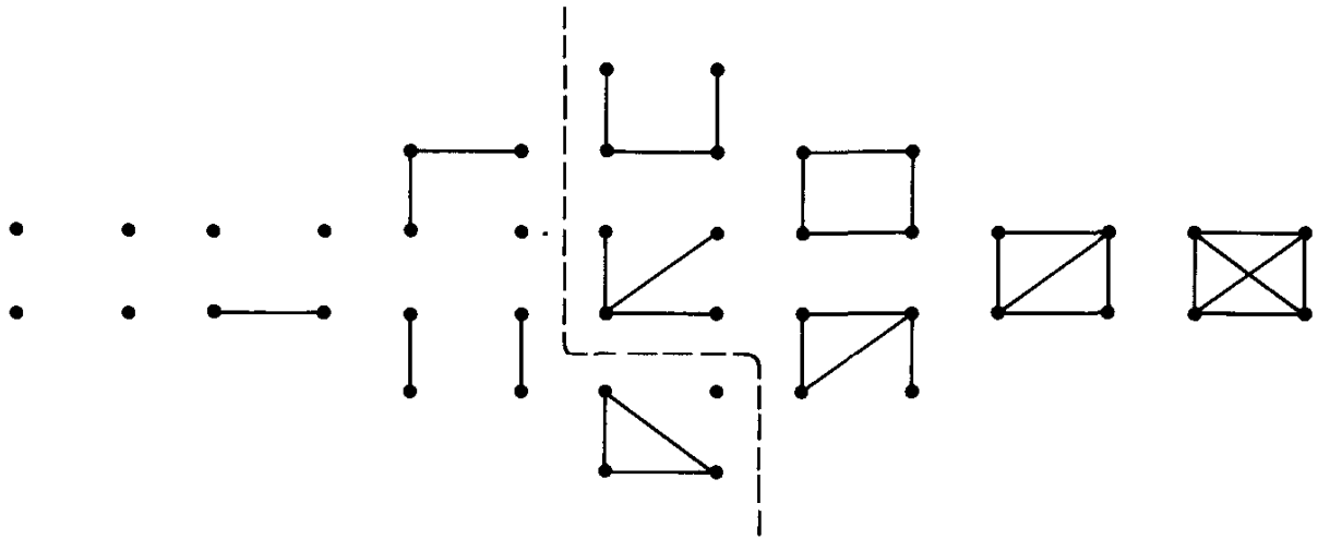
Fig. 2.1. The graphs with four points.
