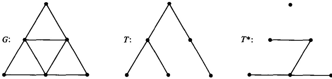
Fig. 4.7. Graph, tree, and cotree.
