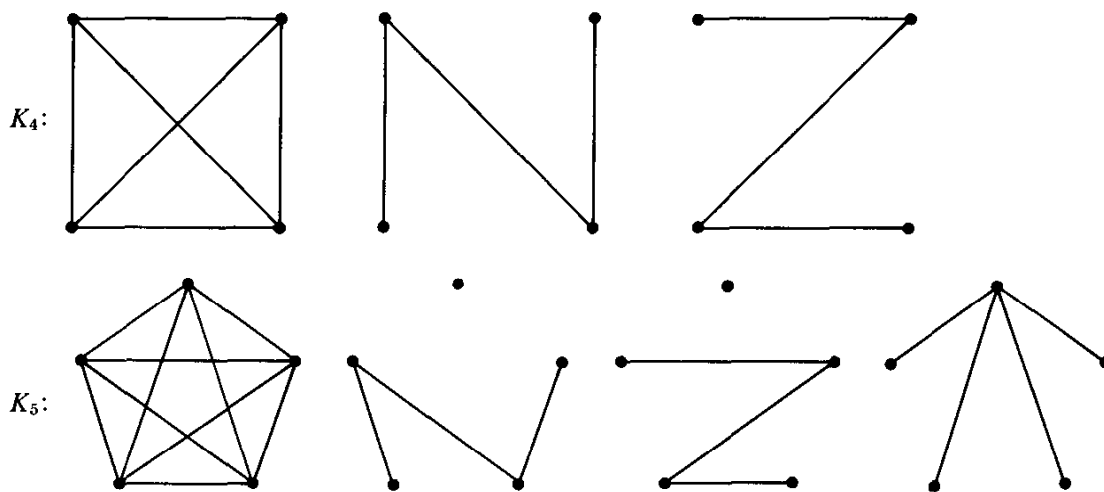
Fig. 9.7. Minimal decompositions into spanning forests.
