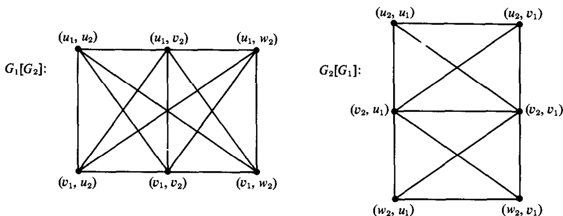
Fig. 2.18. Two compositions of graphs.
