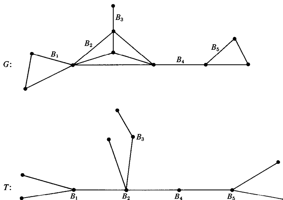
Fig. 8.6. The line-graph G of a tree T .
