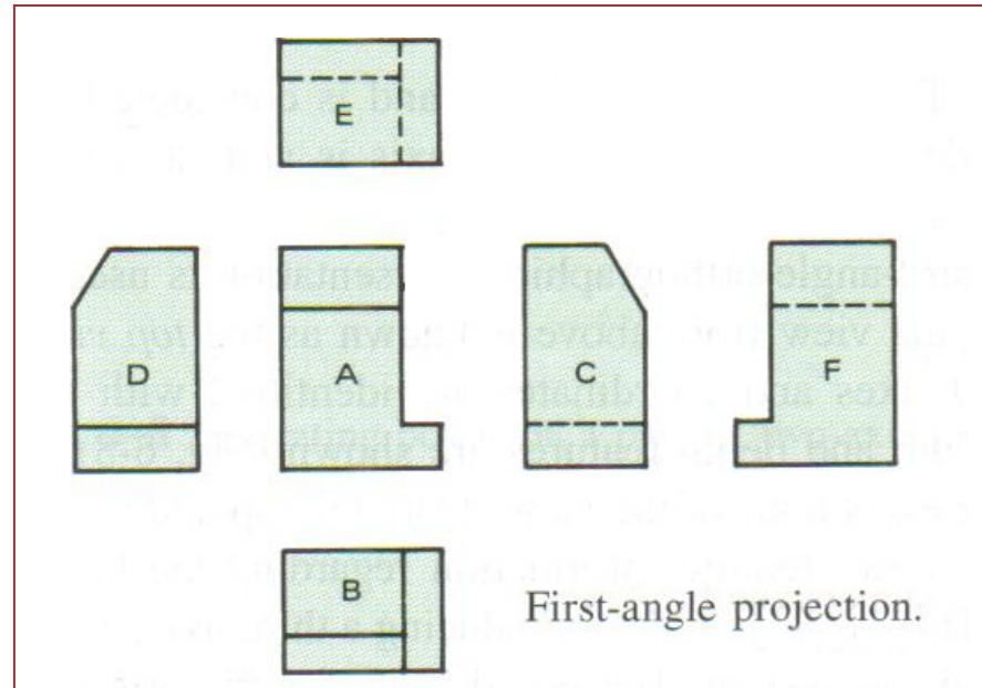
POSITIONING OF VIEWS ON DRAWING SURFACE
