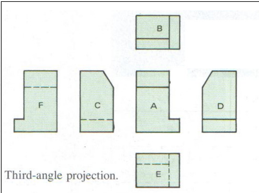
POSITIONING OF VIEWS ON DRAWING SURFACE
