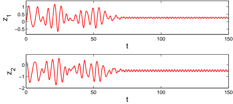
Figure 3: The stabilization of the 2–periodic solution of (5.16) corresponding to the fixed point 3.007/4.007 of the logistic map (5.12). The value \varepsilon = 0.095 is used and the control is switched on at t = \zeta_{20} .
