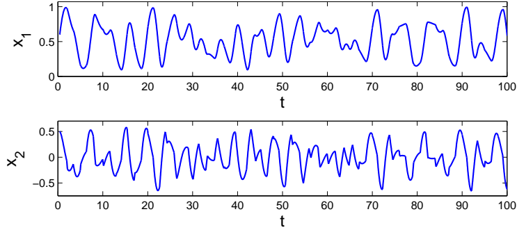
Figure 1: The solution of (5.13) with x_1(0.41) = 0.6 , x_2(0.41) = 0.5 and \kappa_0 = 0.41 . The value \lambda = 4.007 is used in the simulation. The figure reveals the presence of chaos in the dynamics of (5.13).
