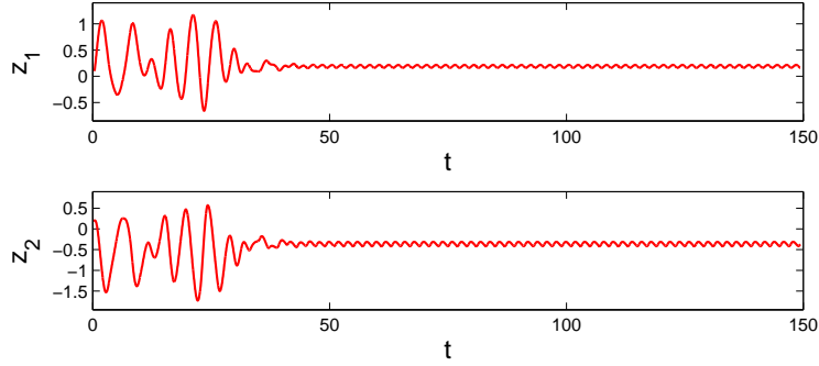
Figure 4: The stabilization of the 2–periodic solution of (5.16) corresponding to the 2–periodic orbit \kappa^{(1)} \approx 0.34459 , \kappa^{(2)} \approx 0.90497 of (5.12). The value \varepsilon = 0.072 is used and the control is switched on at t = \zeta_{25} .
