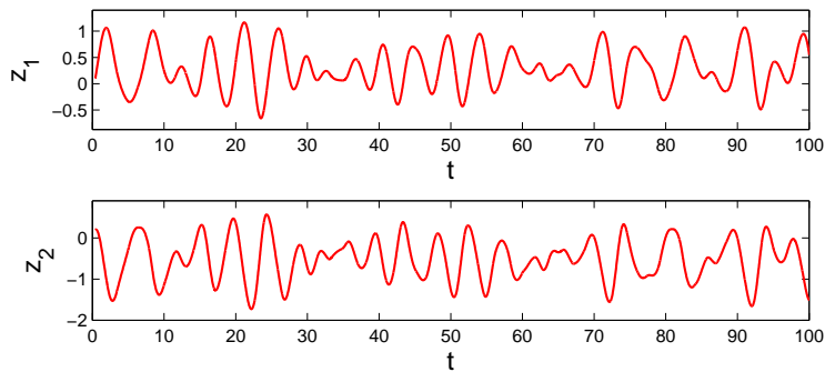
Figure 2: Chaotic behavior in the dynamics of system (5.16). The solution (x_1(t), x_2(t)) represented in Figure 1 is utilized as the perturbation in (5.16). The irregularity is observable in both z_1 and z_2 coordinates.
