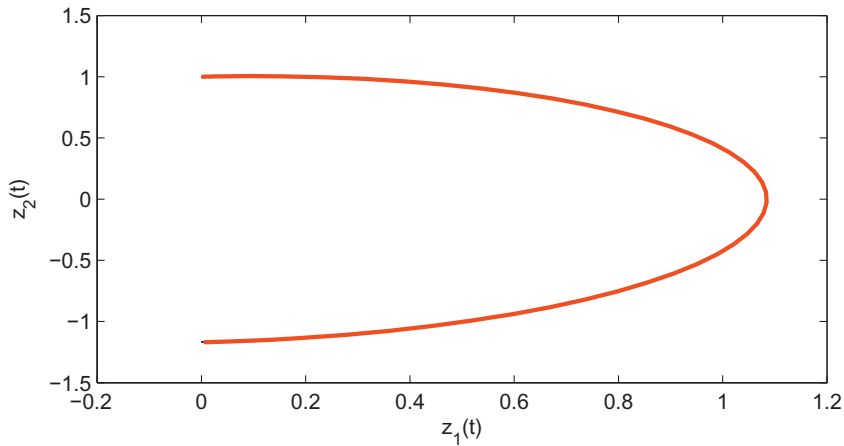
Fig. 2. The grazing orbit of system (3.14).
