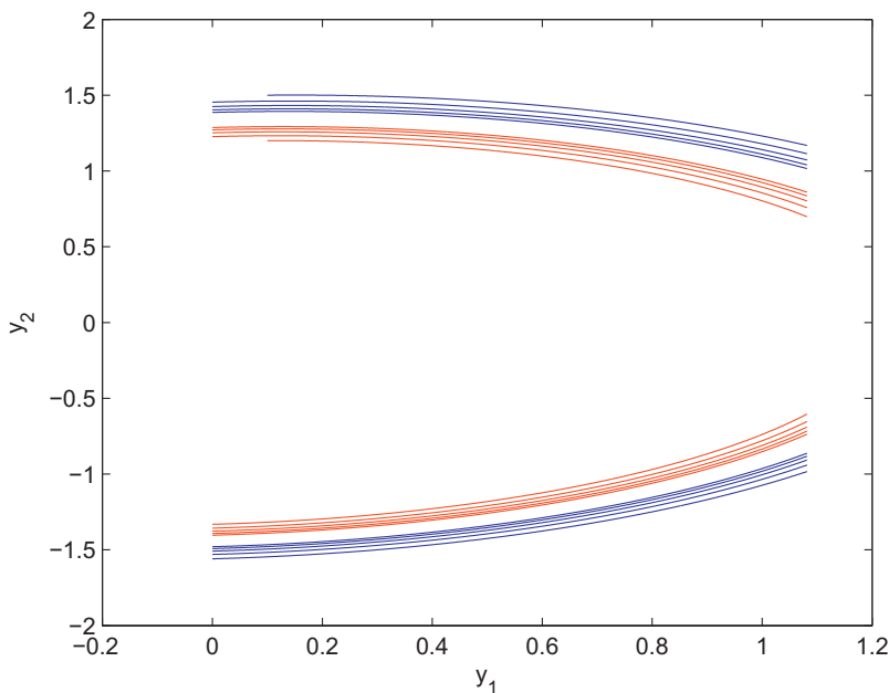
Fig. 7. The red arcs are the trajectory of the system (5.60) with initial value (0, 1.2) and the blue arcs are the orbit with initial value (0, 1.5). Through simulation, we observe that the trajectories approach to the periodic solution of (5.60) as time increases.
