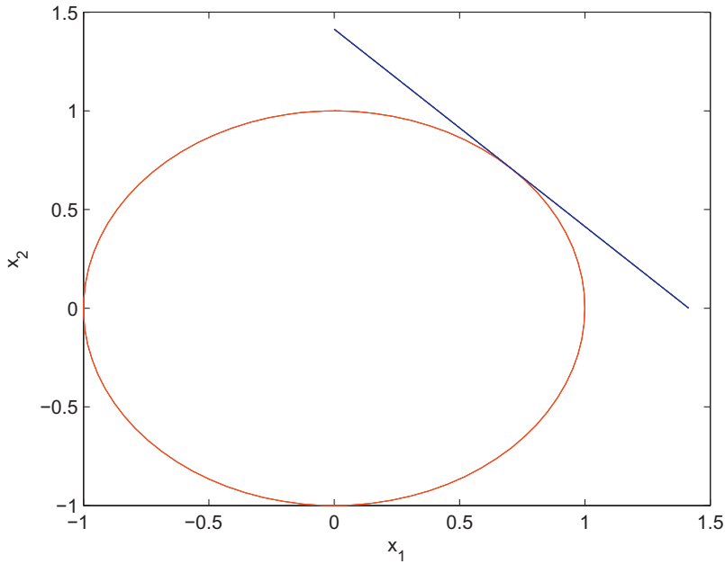
Fig. 5. The red curve is the orbit of \Psi(t) which grazes non-axially the line of discontinuity.
