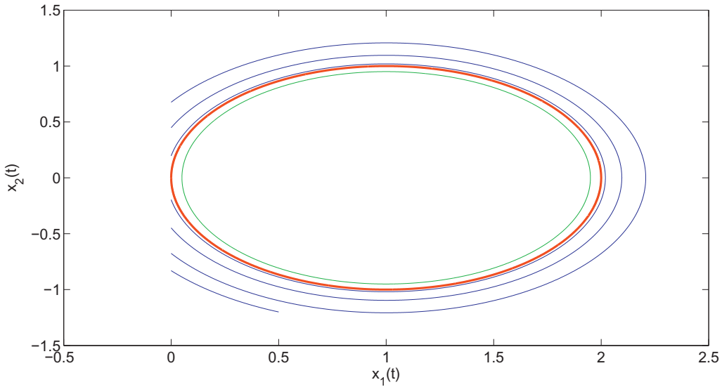
Fig. 8. The grazing cycle of system (5.71) is in red. The blue arcs are the trajectory of the system with initial point (0.5, 1.2) and the green continuous orbit is with initial value (0.1, 0). They demonstrate stability of the grazing solution.
