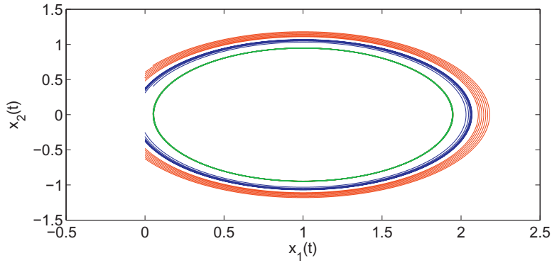
Fig. 9. The blue, red and green arcs constitute the trajectories of system (5.69) with \mu = -0.2 . The first two approach as time increases to the discontinuous limit cycle and the third one is the continuous limit cycle itself. (For interpretation of the references to color in this figure legend, the reader is referred to the web version of this article.)
