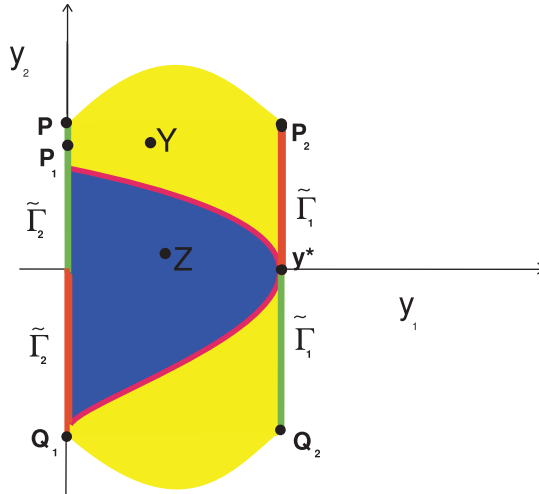
Fig. 1. The region G for system (3.14) is depicted in details. The curves of discontinuity \Gamma = \Gamma_1 \cup \Gamma_2 and \tilde{\Gamma} = \tilde{\Gamma}_1 \cup \tilde{\Gamma}_2 are drawn as vertical lines in red and green, respectively and the grazing orbit in magenta.
