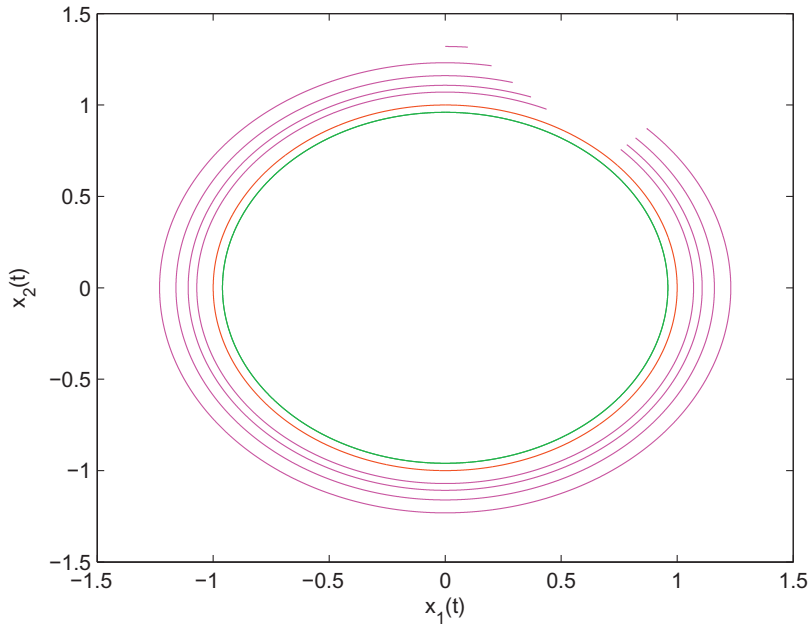
Fig. 6. The red orbit of system (4.50) non-axially grazes the surface \Gamma . The magenta trajectory with initial point (0, 1.32) approaches the cycle as time increases. The green cycle with initial point (0, 0.96) demonstrates the inside stability of the grazing orbit.
