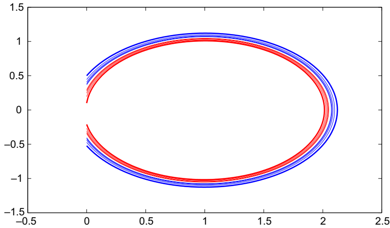
Fig. 10. The red and blue arcs constitute the trajectories of the system (5.69) with \mu = 0.2 . Both orbits approach to the discontinuous limit cycle, as time increases. (For interpretation of the references to color in this figure legend, the reader is referred to the web version of this article.)
