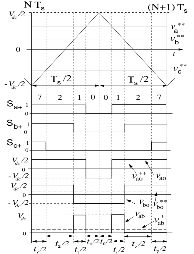
Fig. 5. The per carrier cycle view of switch logic signals, inverter states, and VSI output voltages for 0 \leq w_e t \leq \frac{\pi}{3} ( R = 1 ).
