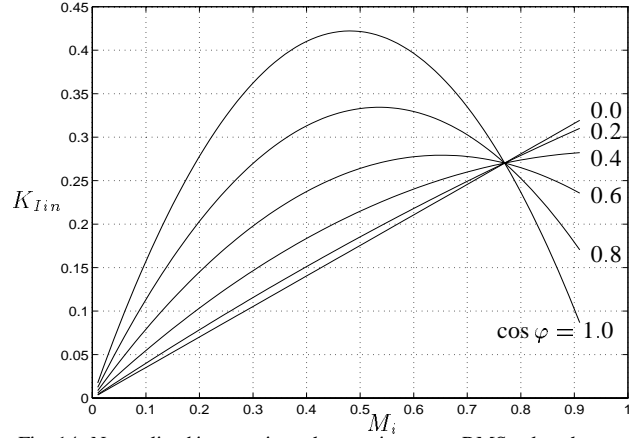
Fig. 14. Normalized inverter input harmonic current RMS value characteristics K_{Iin} = f(M_i) of PWM-VSI for \cos \varphi as parameter.
