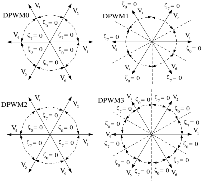
SVPWM: \zeta_0 = \zeta_7 = 0.5 DPWMMAX: \zeta_0 = 0 DPWMMIN: \zeta_7 = 0
