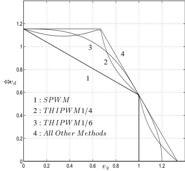
Fig. 19. Vector space illustration of the modulator per carrier cycle voltage linearity limits. All voltage vectors are normalized to \frac{V_{dc}}{2} .
