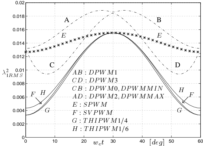
Fig. 12. The space dependency of the per carrier cycle normalized RMS harmonic flux of the modern PWM methods for M_i = 0.78 .
