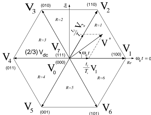
Fig. 3. The space vector diagram illustrates the direct digital implementation principle. The upper switch states are shown in the bracket as (Sa+, Sb+, Sc+) and “1” is “on” state while “0” corresponds to “off” state.
