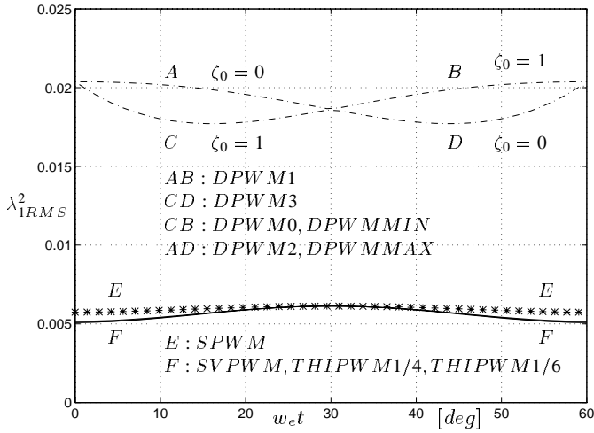
Fig. 11. The space dependency of the per carrier cycle normalized RMS harmonic flux of the modern PWM methods for M_i = 0.4 .
