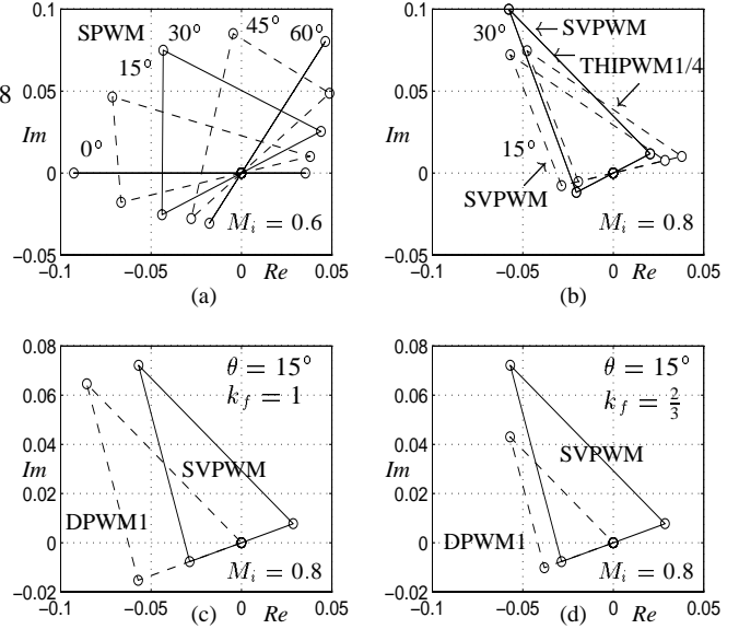
Fig. 10. The switching frequency harmonic flux trajectories of various PWM methods. (a): SPWM, (b): SVPWM and THIPWM1/4 compared for w_e t = 15^\circ and w_e t = 30^\circ values, (c): SVPWM and DPWM1 compared for k_f = 1 , (d): SVPWM and DPWM1 for k_f = \frac{2}{3} .
