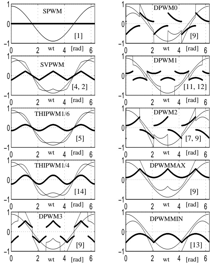
Fig. 6. Modulation waveforms of the modern PWM methods ( M_i = 0.7 ).
