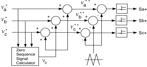
Fig. 4. The generalized signal block diagram of the triangular intersection technique based PWM employing the zero sequence injection principle.
