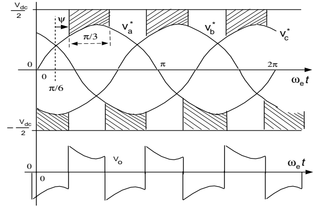
Fig. 7. Generating the GDPWM zero sequence signal with the \psi variable.
