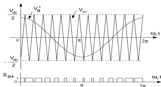
Fig. 2. Triangle intersection PWM phase “a” modulation and switching signals.
