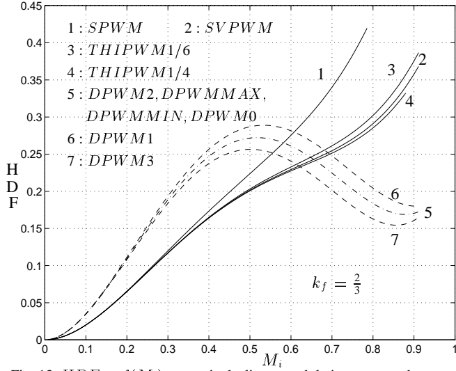
Fig. 13. HDF = f(M_i) curves in the linear modulation range under constant inverter average switching frequency.
