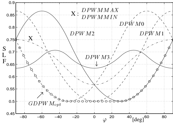
Fig. 17. SLF = f(\varphi) characteristics of the modern DPWM methods under fixed carrier frequency constraint ( SLF_{CPWM} = 1 ).
